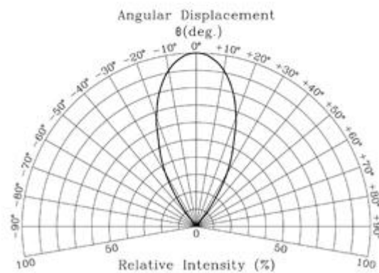
Relative Radiant Intensity & Angular Displacement
